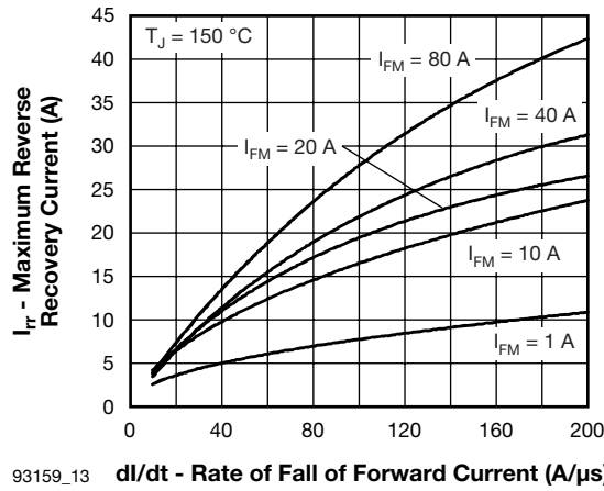
93159_13 di/dt - Rate of Fall of Forward Current ( \text{A}/\mu\text{s} ) Fig. 13 - Recovery Current Characteristics, T_J = 150^\circ\text{C}
