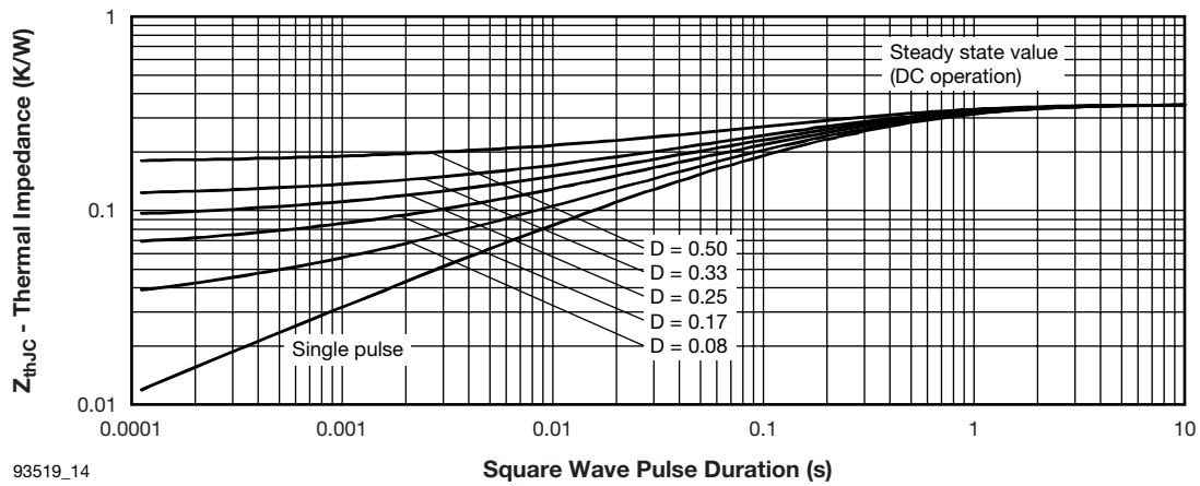
93519_14 Fig. 14 - Thermal Impedance Z_{thJC} Characteristics
